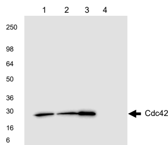
Figure 1: Western Blot: Demonstration of ACD04 sensitivity & specificity
